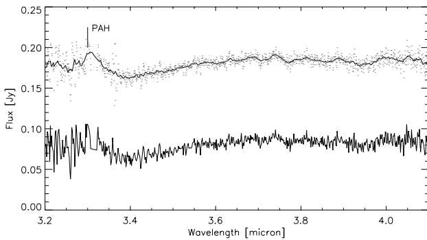
Fig. 8. The spectrum of SMC-S2, and smoothed spectrum to 1/10th of the original wavelength resolution. The 3.3 \mu\text{m} PAH band is detected. (The 3.308\text{--}3.320 \mu\text{m} region is removed because of strong telluric lines.) 10\sigma errors are plotted as dots.
